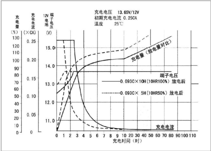
Charge Characteristics Constant Voltage with Current Limit
